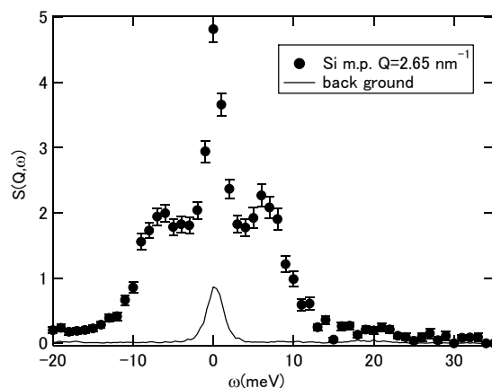
Fig.3 S(Q, \omega ) of liquid Si at m.p.
