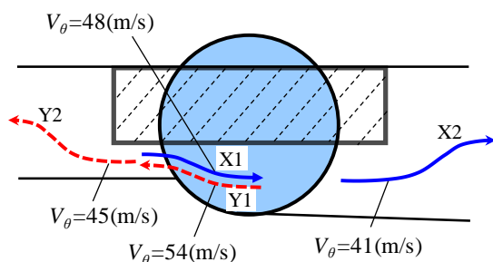
Fig.8 Meridional flow and rotational speed
