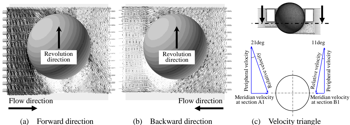
Fig.5 Velocity vector around bearing ball at 40000rpm
