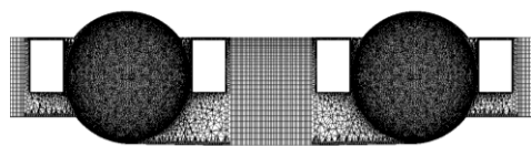
(c) Grid of matched mounting bearing
