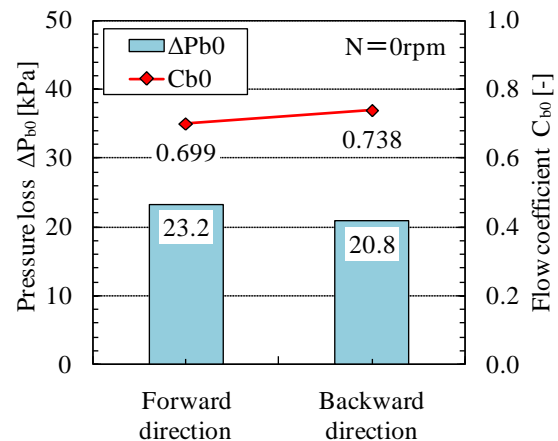
Fig.4 Comparison of pressure losses between flow directions at 0 rpm
