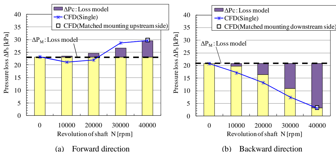
Fig.9 Estimation of pressure loss (coolant flow rate = constant)
