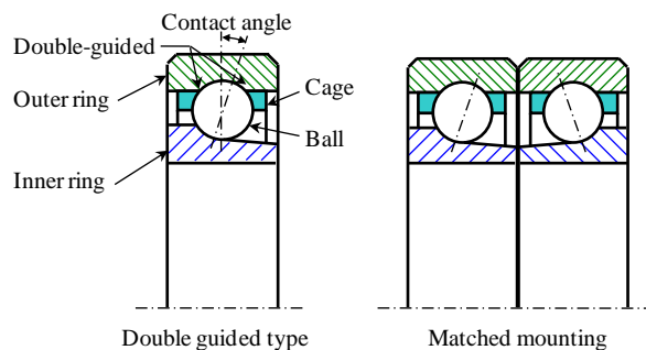
Fig.1 Angular contact ball bearing
