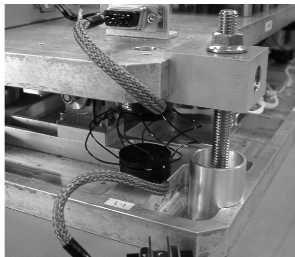
Fig.5 The improved damper and Model 2001.
