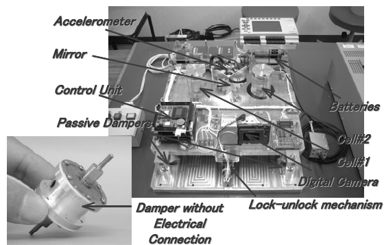
Fig.3 The damper and the apparatus(Model 2001).
