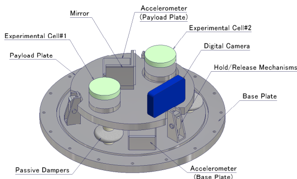
Fig.8 The new concept (Model 2005)
