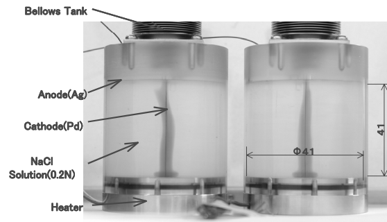
Fig.1 The experimental cells using electrical color development
