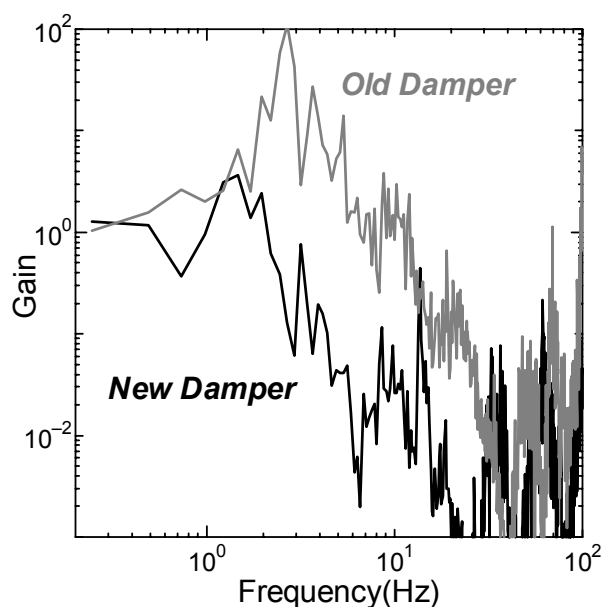
Fig.6 The comparison of isolation performance between new and old dampers.
