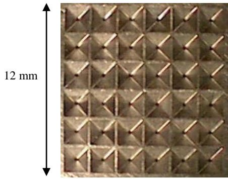
Fig.3 Photos of expansion 36 nozzles.
