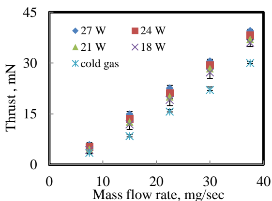
Fig.11 Thrust vs mass flow rate of nozzle performance.
