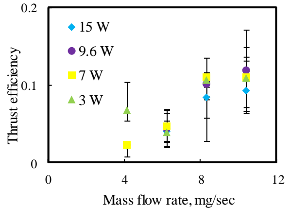
Fig.9 Thrust efficiency vs mass flow rate for comparison of nozzle performance.
