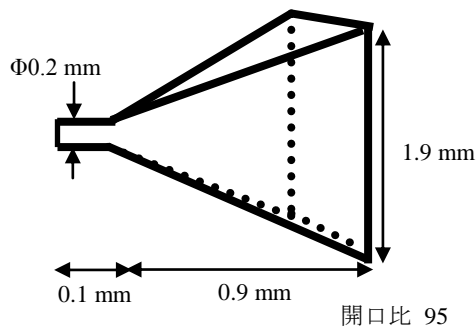
Fig.5 Schematic of 1 nozzle.
