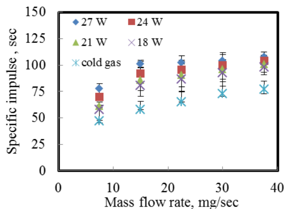
Fig.12 Specific impulse vs mass flow rate for comparison of nozzle performance.
