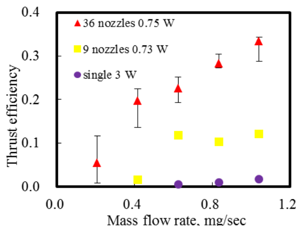
Fig.16 Thrust efficiency vs mass flow rate for comparison of nozzle performance.
