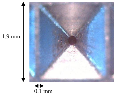
Fig.4 Photo of expansion 1 nozzle of 36 nozzles.
