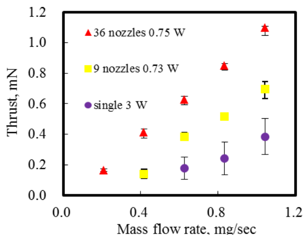
Fig.14 Thrust vs mass flow rate for comparison of nozzle performance.
