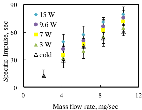
Fig.8 Specific impulse vs mass flow of nozzle performance.
