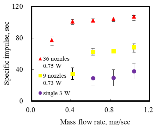
Fig.15 Specific impulse vs mass flow rate for comparison of nozzle performance.
