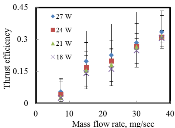
Fig.13 Thrust efficiency vs mass flow rate for comparison of nozzle performance.
