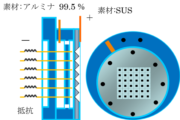
Fig.2 Isolation of each electrode array thruster.
