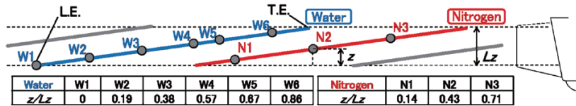
Fig. 3 Development view of the inducer showing location of pressure sensors for measurements of pressure rise
