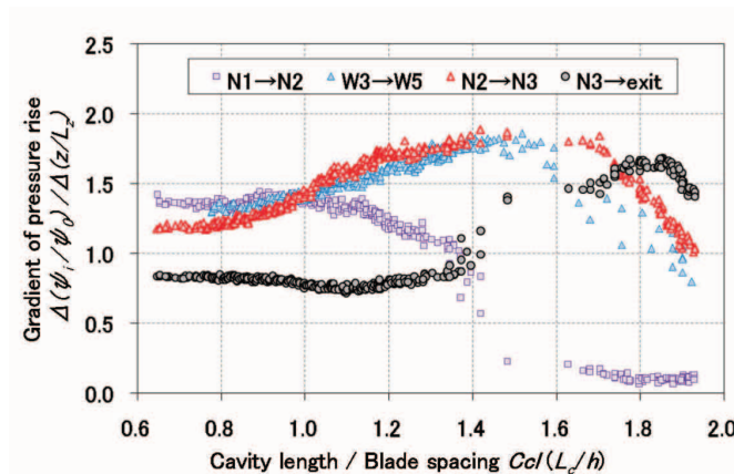
Fig. 8 Comparison of the gradient of pressure rise between liquid nitrogen and water
