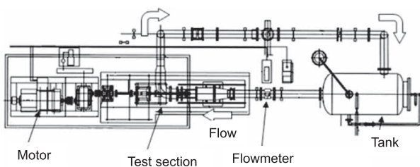
Fig. 1 Inducer Test Facility of IHI
