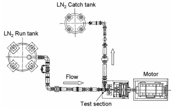
Fig. 2 Cryogenic inducer test facility of JAXA
