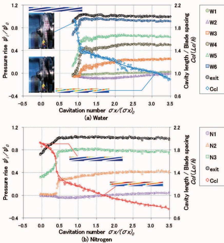
Fig. 7 Pressure rise and cavity length in cold water ( upper ) and in liquid nitrogen ( lower )
