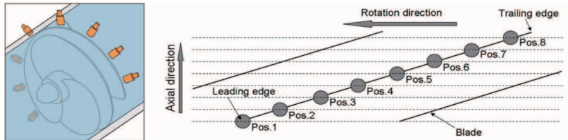
Fig. 4 Location of pressure taps along the blade for measurements of unsteady pressure
