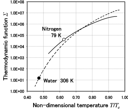
Fig. 6 Comparison of the thermodynamic function \Sigma(T) of nitrogen and water
