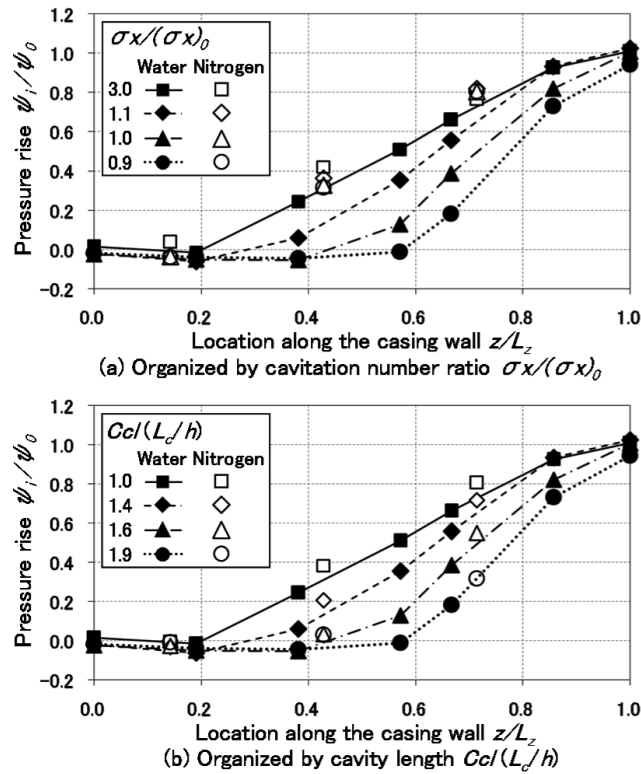
Fig. 9 Pressure rise along the tip organized by cavitation number and cavity length
