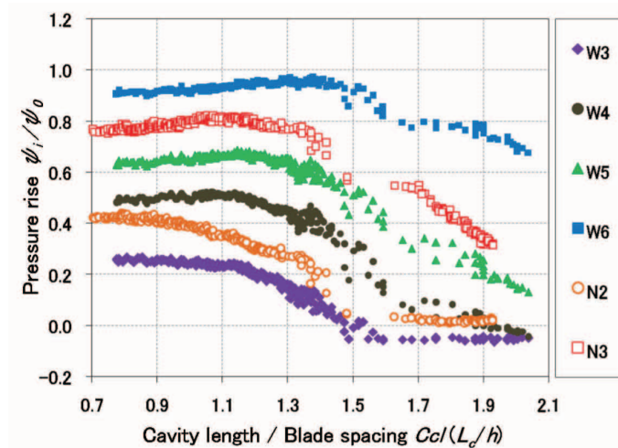
Fig. 10 Comparison of the change of pressure rise between in liquid nitrogen and water
