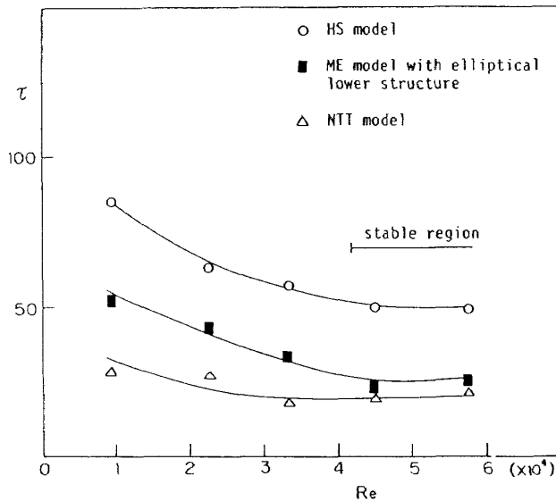
Figure 2. Flushing time parameter (Reynolds number effect)
