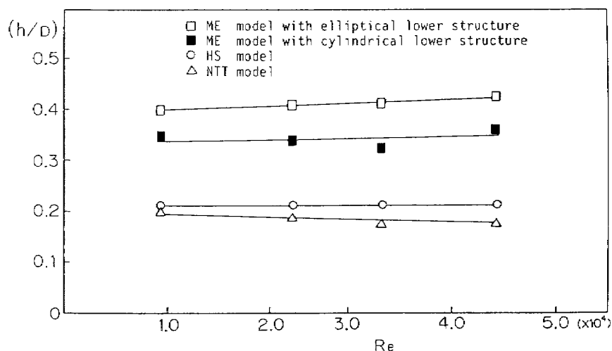
Figure 5. Containing flow height (Reynolds number effect)
