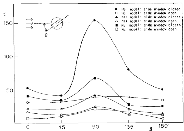
Figure 11. Flushing time parameter (orientation angle effect)
