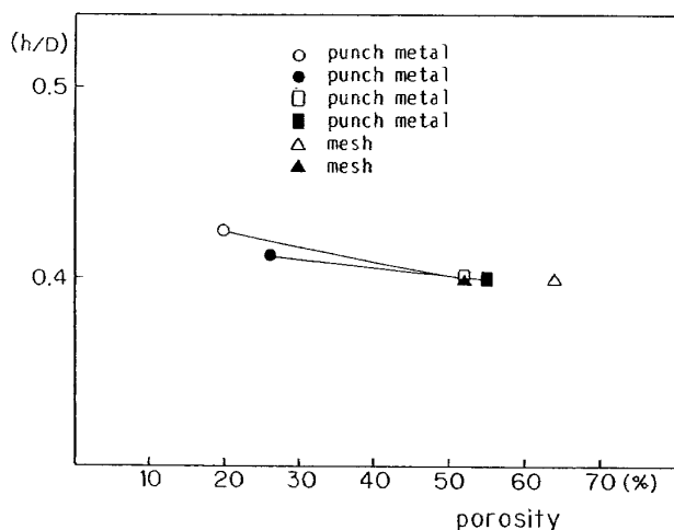
Figure 6. Windscreen porosity effect to containing flow height
