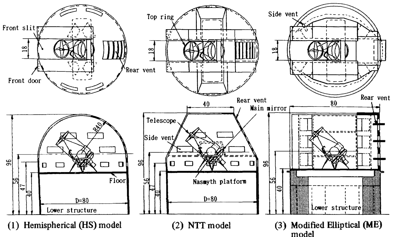
Figure 3. The three telescope enclosure models
