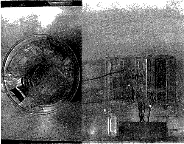
Figure 12. Flow pattern of the ME style (45°)
