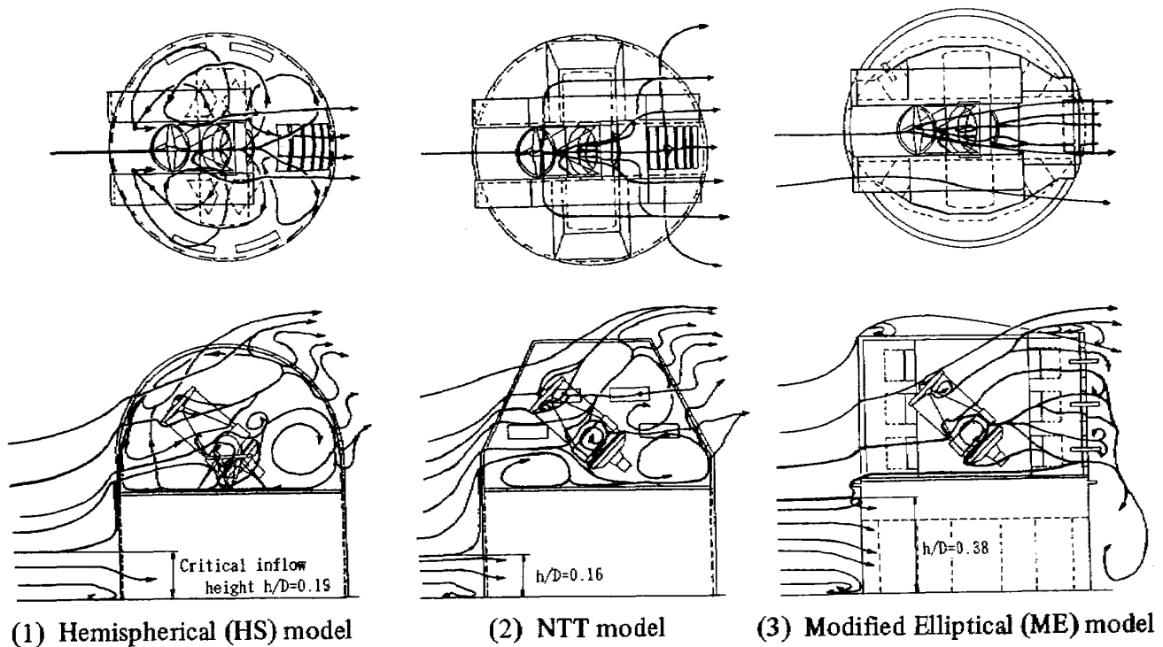
Figure 10. Sketch of typical flow patterns of inside and outside of the enclosures
