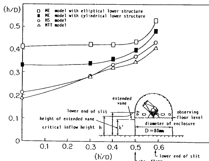
Figure 7. Extended vane height to containing flow height
