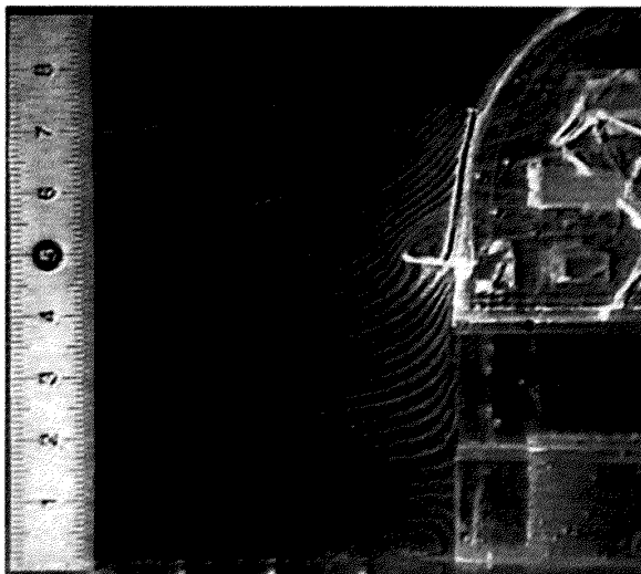
Figure 8. Photograph of extended vane height effect
