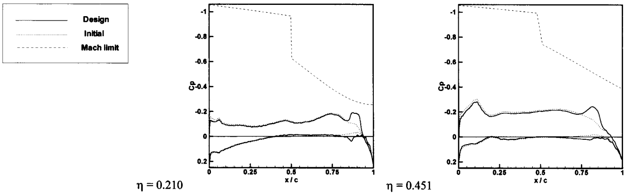
Fig.7 LE & TE design results with inboard flap deflection activated; Surface pressure distributions for inboard sections
