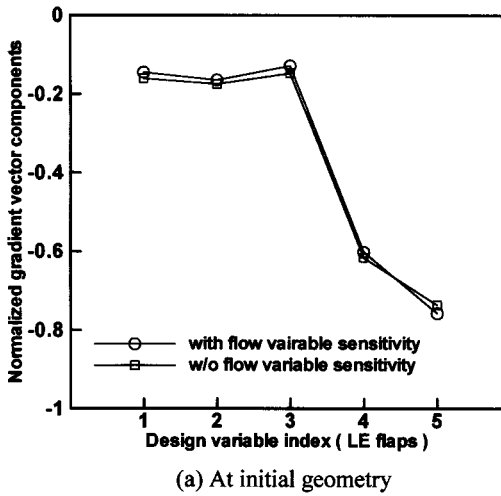
Fig.3 Comparison of sensitivity derivatives for initial geometry
