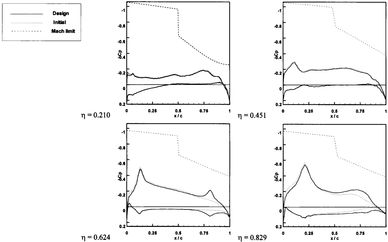
Fig.8 LE & TE design results with inboard flap not activated; Surface pressure distributions
