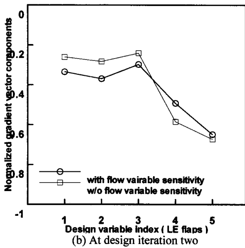
Fig.4 Comparison of normalized sensitivity derivatives
