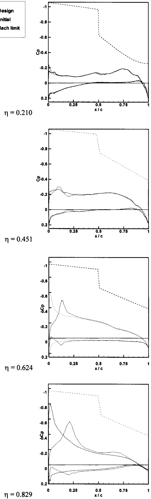
Fig.5 Wing section surface pressure distributions (design I by AGE)
