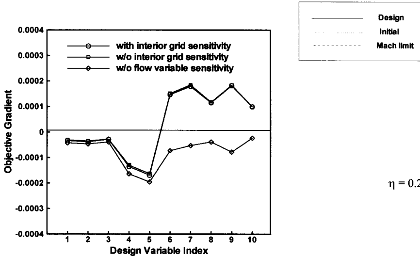
Fig.3 Comparison of sensitivity derivatives for initial geometry
