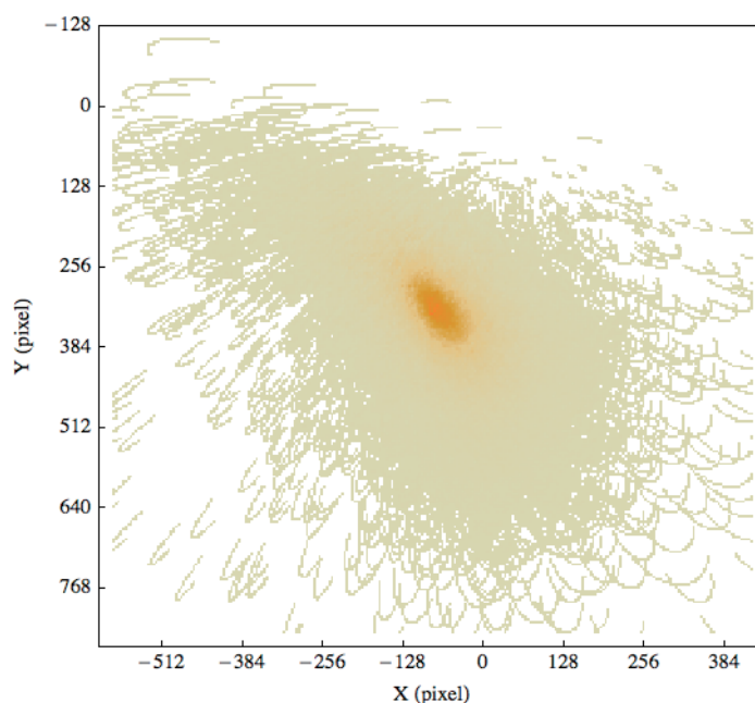
Fig. 4. Distribution of Two-dimensional Shift Values of US Titan IIIC Transtage Fragments in Successive Images
