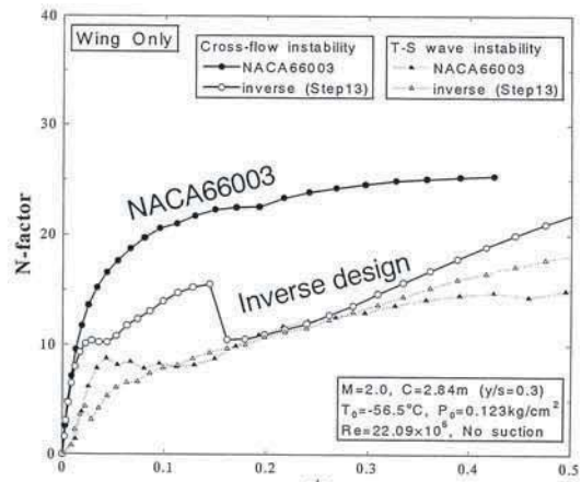
Fig.4 Results of boundary layer stability analysis.
