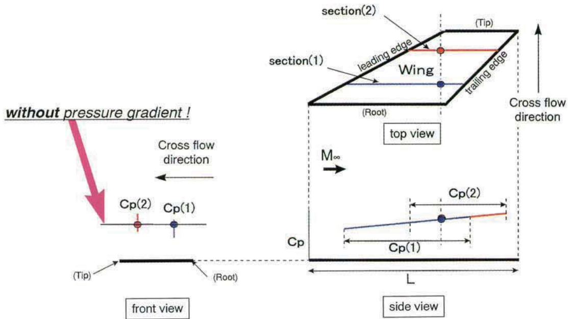
Fig.6 A model of spanwise pressure distribution of new NLF concept wing
