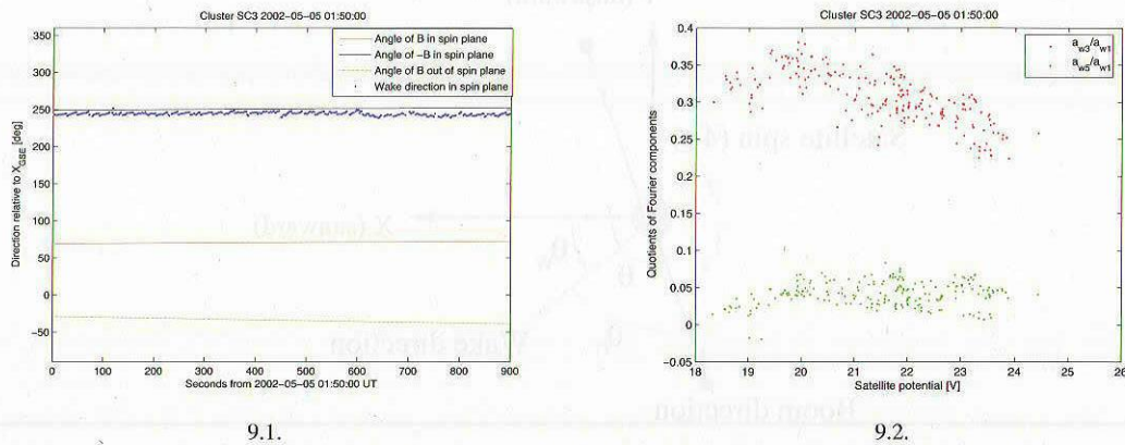
Fig. 9. 1. Angles versus time: Derived angles of the wake (blue), \alpha = 360 \text{ deg} - \angle(X_{\text{GSE}}, \mathbf{B}) in spin plane (red), \alpha + 180 \text{ deg} (black), and elevation angle of \mathbf{B} out of the spin plane. 2. Dependence of the wake Fourier components on the satellite potential. Red dots corresponds to a_{w3}/a_{w1} , while green dots represents a_{w5}/a_{w1} .
