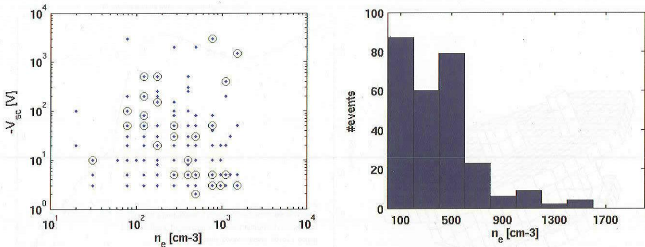
Fig. 6. Left : Charging level vs. plasma density. Rings mark charging events in sunlight. Right : Distribution of plasma densities in charging events, with bins centred on 100, 300, 500, ... \text{cm}^{-3} .
