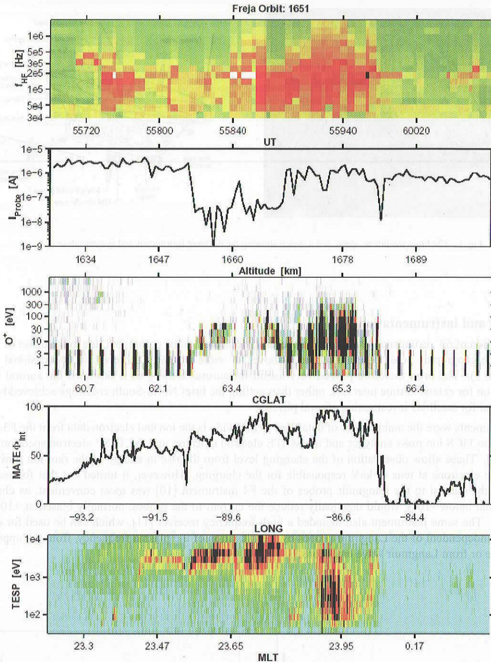
Fig. 3. An example event in the auroral zone. Panels from top to bottom: (i) Wave activity from 30 kHz to 2 MHz. (ii) Current to a Langmuir probe, biased to +10 V. (iii) Ion spectrogram up to 3 keV. (iv) Integrated flux of electrons 5 keV – 100 keV (uncalibrated). (v) Electron spectrogram up to 10 keV. Similar plots for all Freja charging events are available at http://www.ava.fmi.fi/spee/freja.html .
