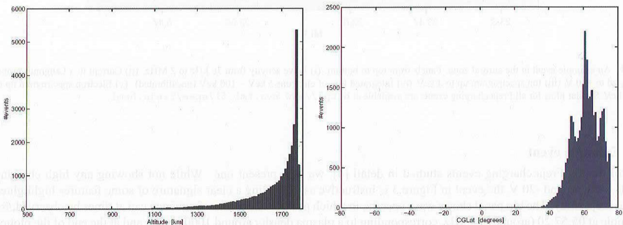
Fig. 2. The Freja coverage coverage of altitudes (left) and corrected geomagnetic latitudes (right) during its almost three years of operational lifetime. The histograms were made by dividing each ground station pass (15 – 30 minutes) into four intervals, using the positions at their centres.
