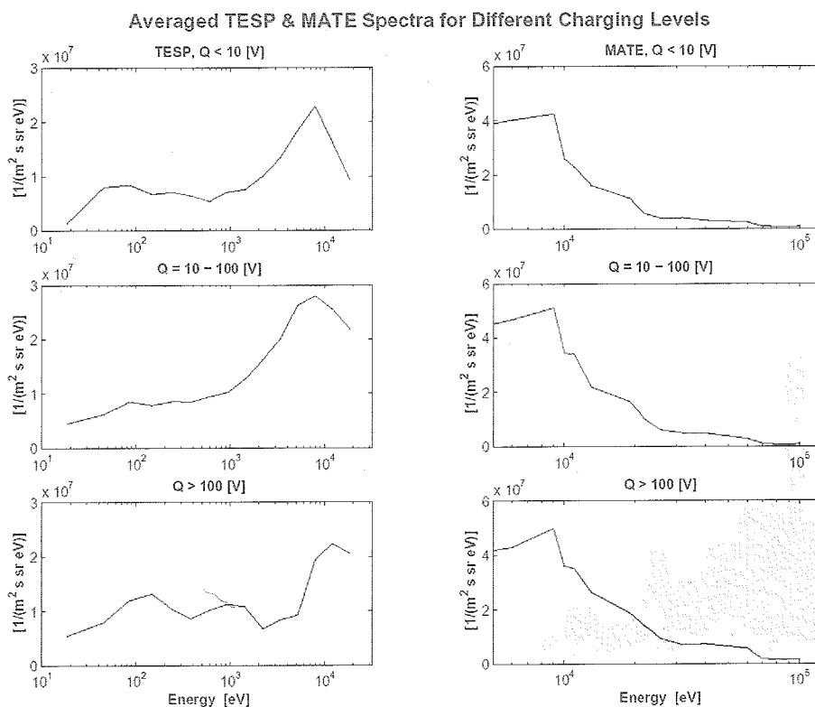
Fig. 5. Averages of all electron spectra obtained during charging events by the two electron detectors TESP [9] and MATE [8], sorted by the magnitude of the charging level, Q .
