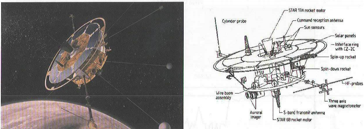
Fig. 1. The Freja satellite in space, and a sketch showing the different instruments and system sub-units.
