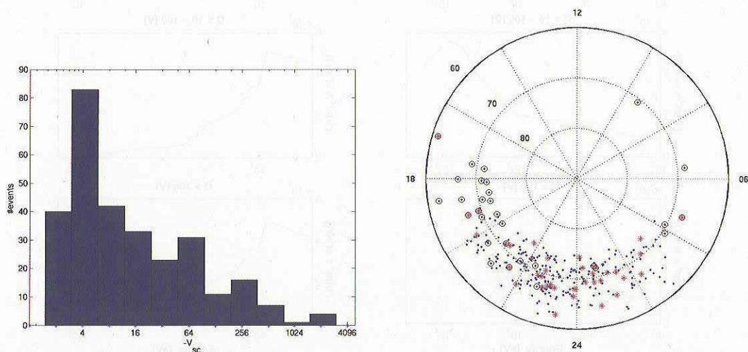
Fig. 4. Left : Histogram showing the charging voltage in the Freja charging events, binned in logarithmically spaced intervals. Right : Polar plot illustrating their distribution in geomagnetic coordinates. Red stars mark events charged below -100 V, and rings denote events in sunlight.
