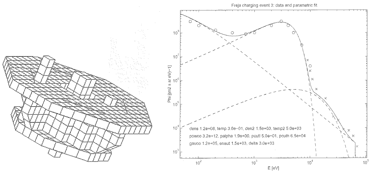
Fig. 7. Left : The most complete Freja model used in the POLAR simulations, with 10 cm grid resolution. Right : Observed and fitted electron spectra for modelling with POLAR. Circles are data from the TESP detector, crosses from MATE (Section 3). The fitted curve has been mapped through the observed spacecraft potential to correct for effects of the charging event.
