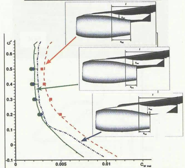
Fig. 18 Prediction of engine-airframe interference drag using the TAU-Code, (a) hybrid grid for DLR-F6 configuration, (b) lift as a function of installation drag for three different position of CFM56 engine, M_\infty=0.75 , Re=3 \times 10^6 , symbols: calculation, lines: experiment.
